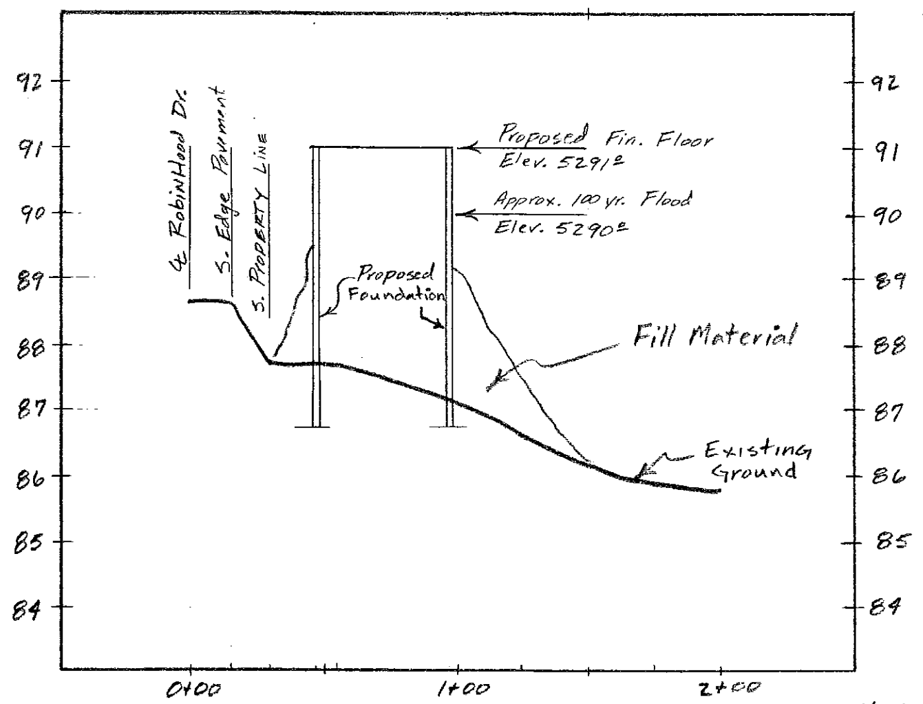
PROFILE - LOT
