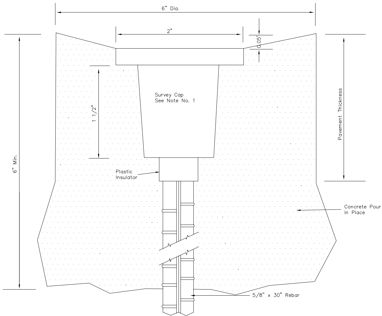
TYPICAL SECTION SURVEY CAP FOR REBAR (TYPE I) N.T.S.
