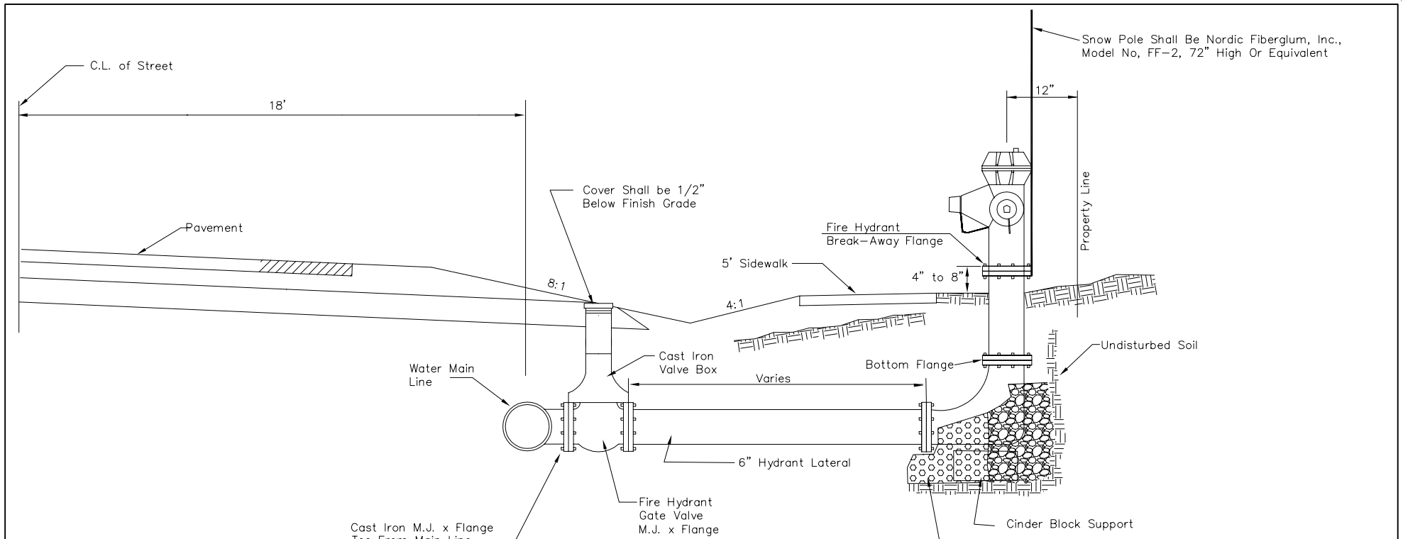
TYPICAL SECTION FIRE HYDRANT ASSEMBLY RESIDENTIAL STREET OPTION 2 N.T.S.
