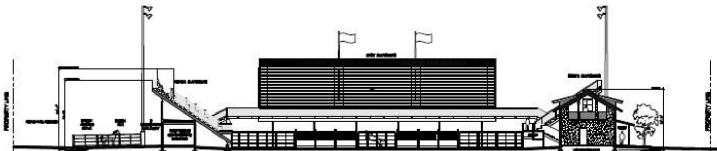
SECTION 1 / ELEVATION - BLEACHERS AND VISITOR CENTER LOOKING EAST
